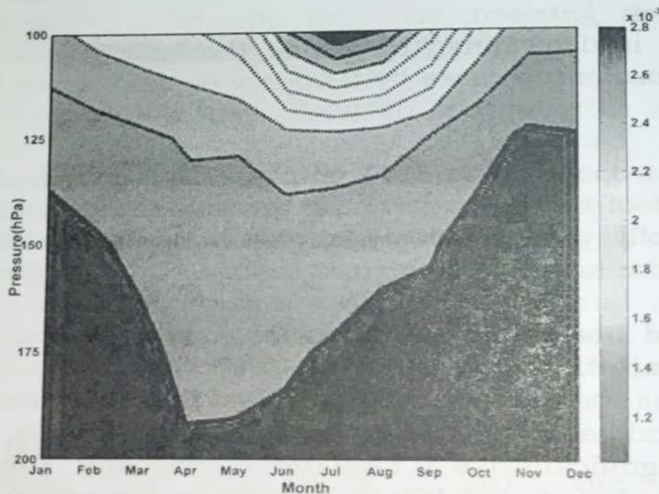
Fig.1.1. Seasonal variation of ozone mixing ratio (kg/kg) in 100-200 hPa layer for 0°N to 20°N and 60°E to 100°N.
