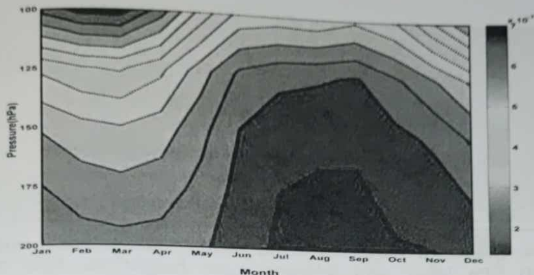
Fig .1.2. Seasonal variation of ozone mixing ratios (kg/kg)in 100-200 hPa layer for 20°N to 40°N and 60°E to 100°N.
